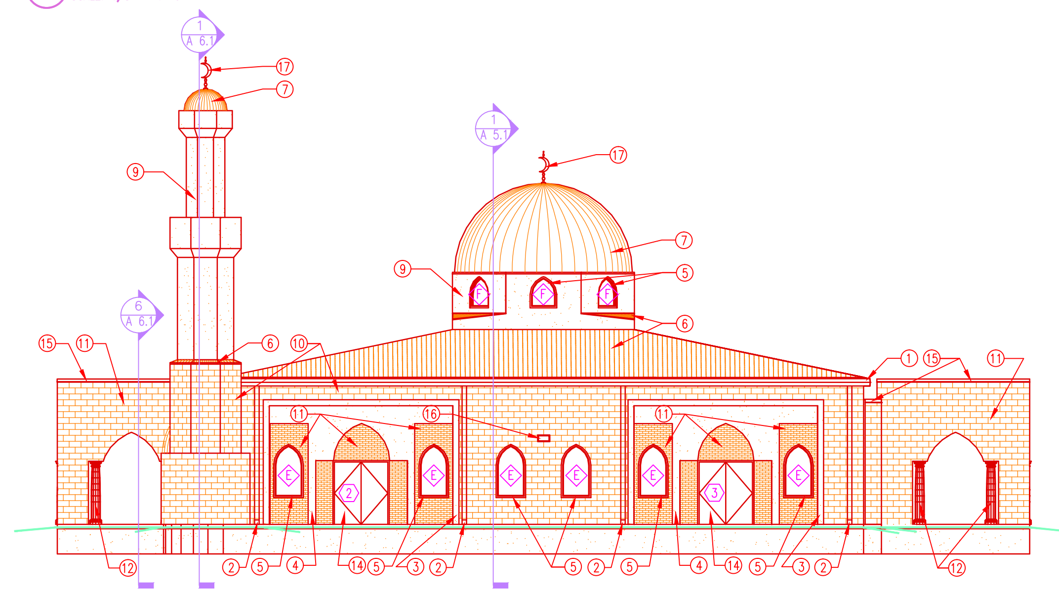
2 WEST ELEVATION SCALE: 3/32" = 1'-0"
