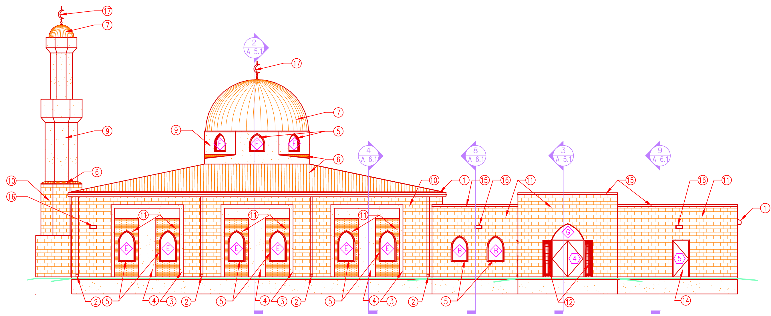
3 SOUTH ELEVATION SCALE: 3/32" = 1'-0"
